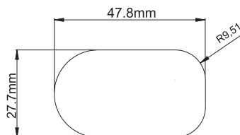
Battery Box Opening Hole Drawing
