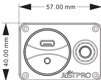
18650 Battery Box
