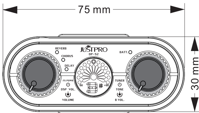
Preamplifier
