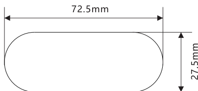
Preamplifier Opening Hole Drawing
